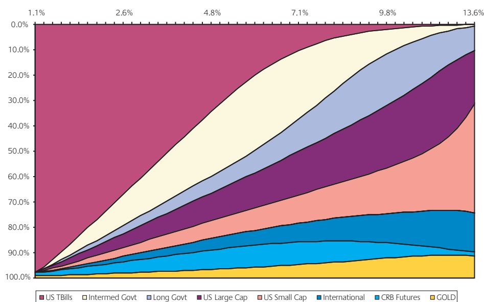
Chart 6: Base case with gold and commodities, January 1974-December 2005
