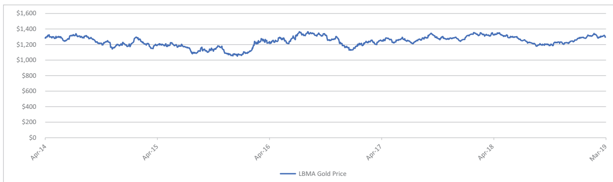
Daily gold price – April 1, 2014 to March 31, 2019
